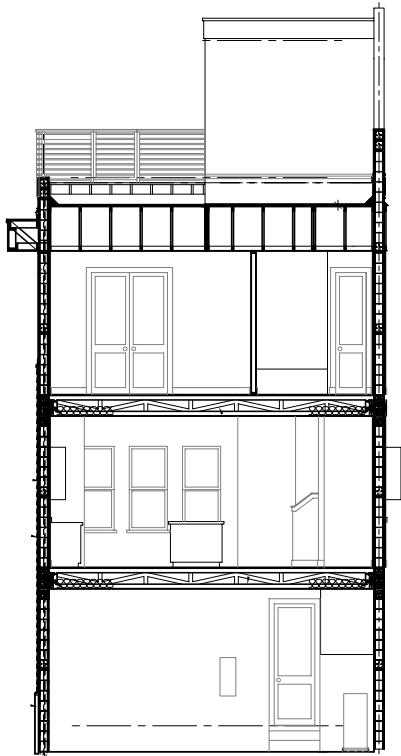
UNIT 5 ELEVATION
