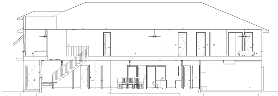
CROSS SECTION #2
